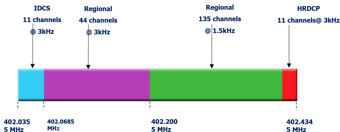
Figure 2 Allocation of International/Regional DCP Channels
