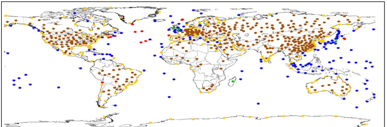
Figure 2: Global location of radiosondes collocated with at least one satellite observation platform for a 2-day period during January 2009; colors indicate the terrain flag of the radiosonde (red, ship; brown, land; yellow, coast; blue, island and green, inland island)
