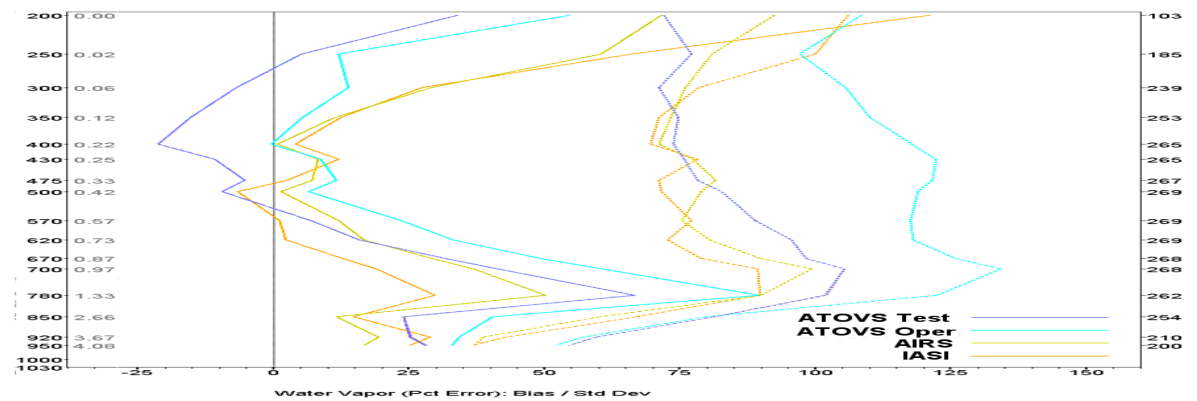
Figure 7b: ATOVS and hyper-spectral satellite-minus-raob H 2 O vapor fractional (%) mean and standard deviation differences using raobs with H 2 O profile scores of 2 or more.
