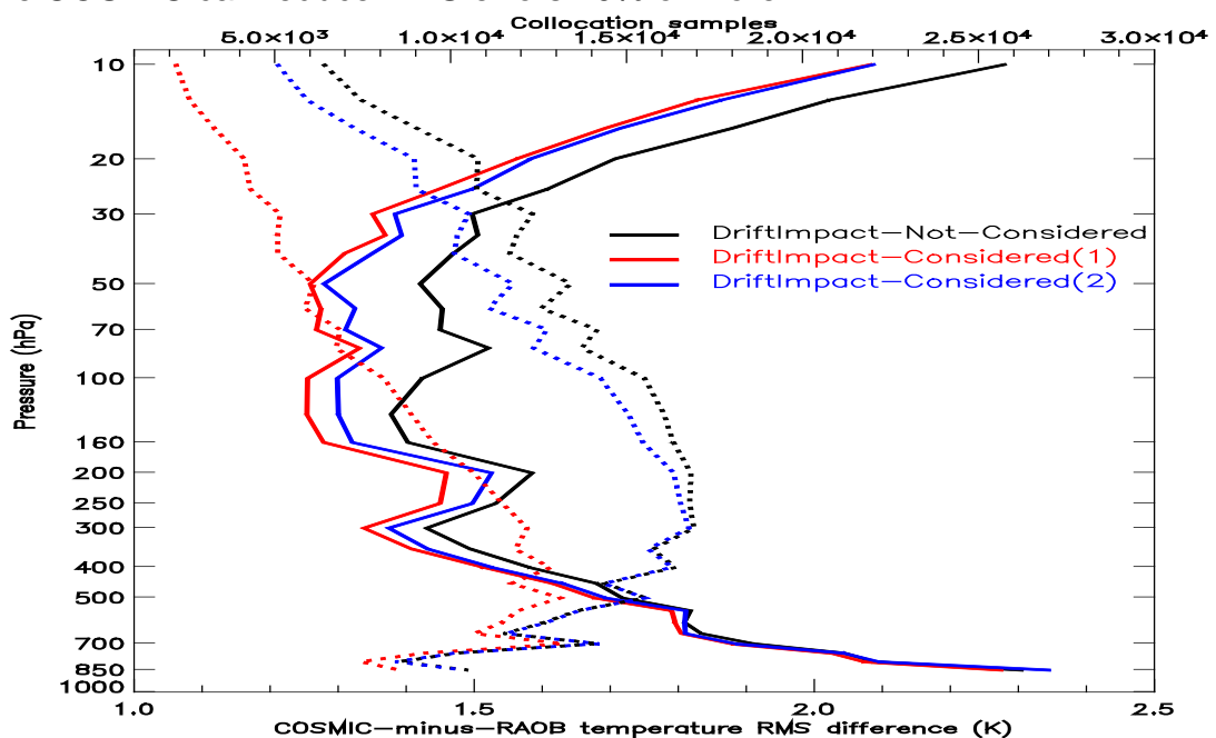
Figure 9: Reduction in Raob-minus-COSMIC RMS (solid) when drift parameters are used (red and blue) to compile collocation samples (dashed) at each vertical level (Sun et al. 2009) with sample size along the top axis and pressure (1000 mb to 10 mb) along the left axis.
