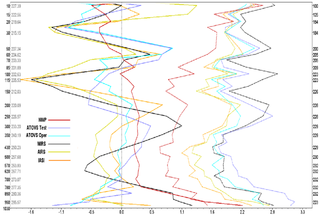
Figure 10: Mean and standard deviation differences for NOAA NWP (red) and five (5) independent suites of temperature soundings-minus-Raob for the period February 8-14, 2009 using common denominator sample (right axis) over sea with pressure (1000 mb to 10 mb) along the left axis.
