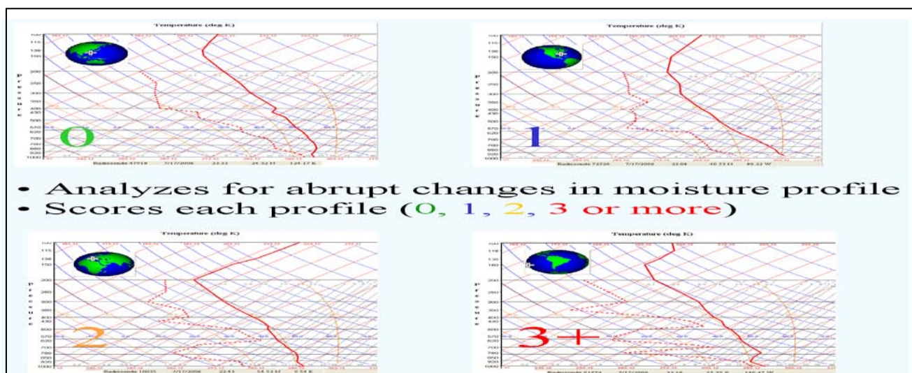
Figure 4: Raob moisture profile (dashed) scores.
