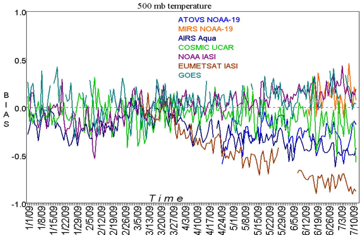
Figure 11: Trend plots of mean Sat-minus-Raob 500mb temperature (+/- 1.0K) for denoted Sat systems during January to July 2009
