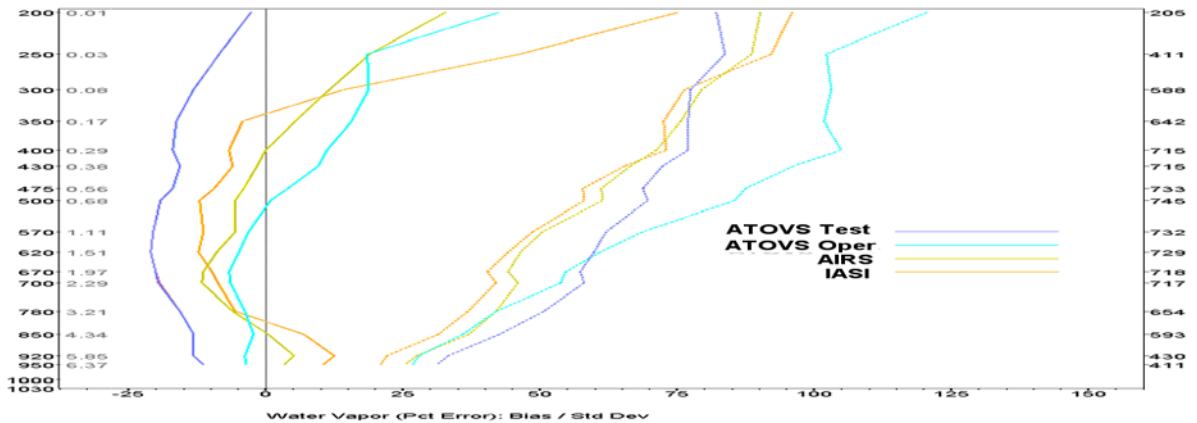
Figure 7a: ATOVS and hyper-spectral Sat-minus-Raob H 2 O fraction (%) mean and standard deviation differences using Raobs with H 2 O profile scores of 0 or 1.
