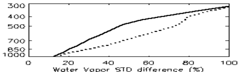
Figure 5: Raob-minus-NWP H 2 O vapor fractional (%) differences for Raobs with moisture scores 0,1 (solid) and 2 or more (dashed).
