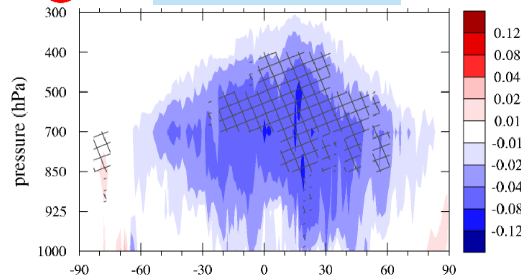
Specific humidity (g/kg)
