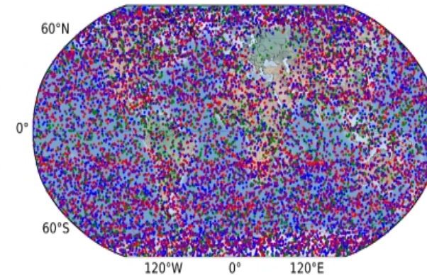
GPS BDS GLONASS GALILEO
