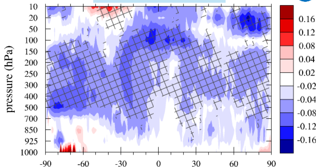
Wind speed (m/s)
