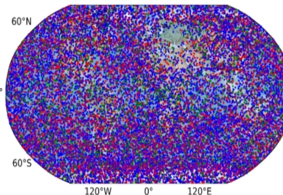
GPS BDS GLONASS GALILEO
