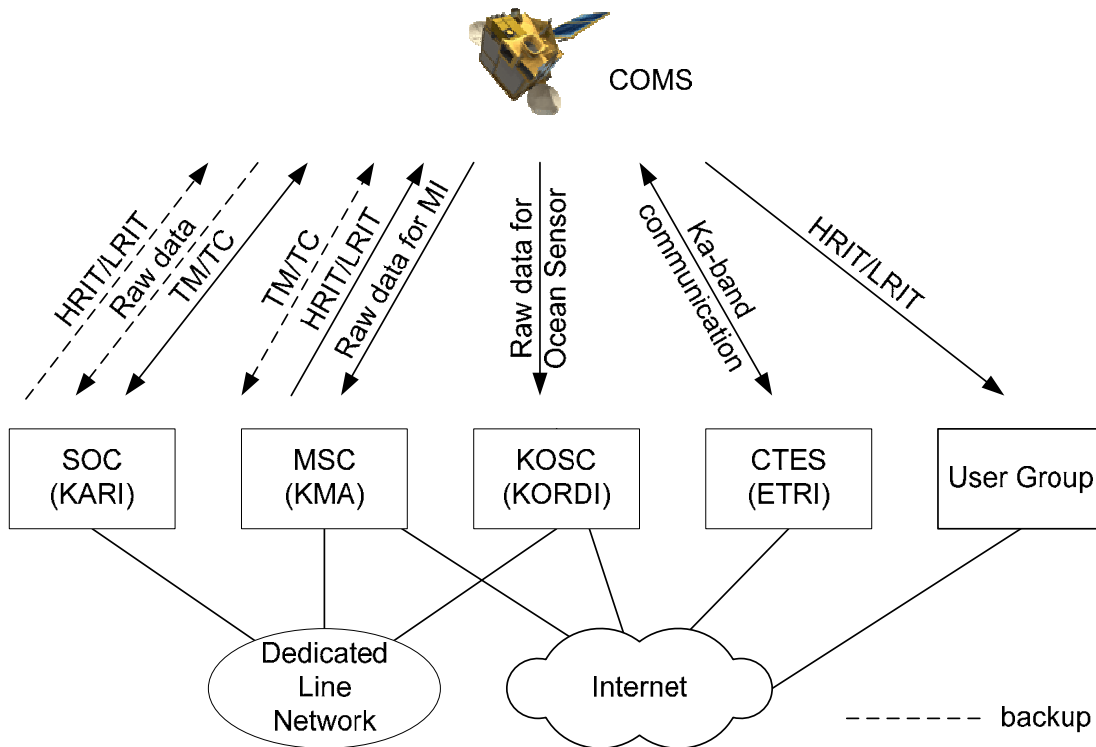
Figure 1 COMS ground segment architecture
