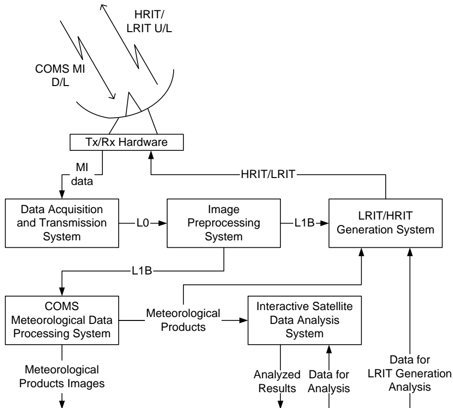
Figure 2 Functional components of COMPASS
