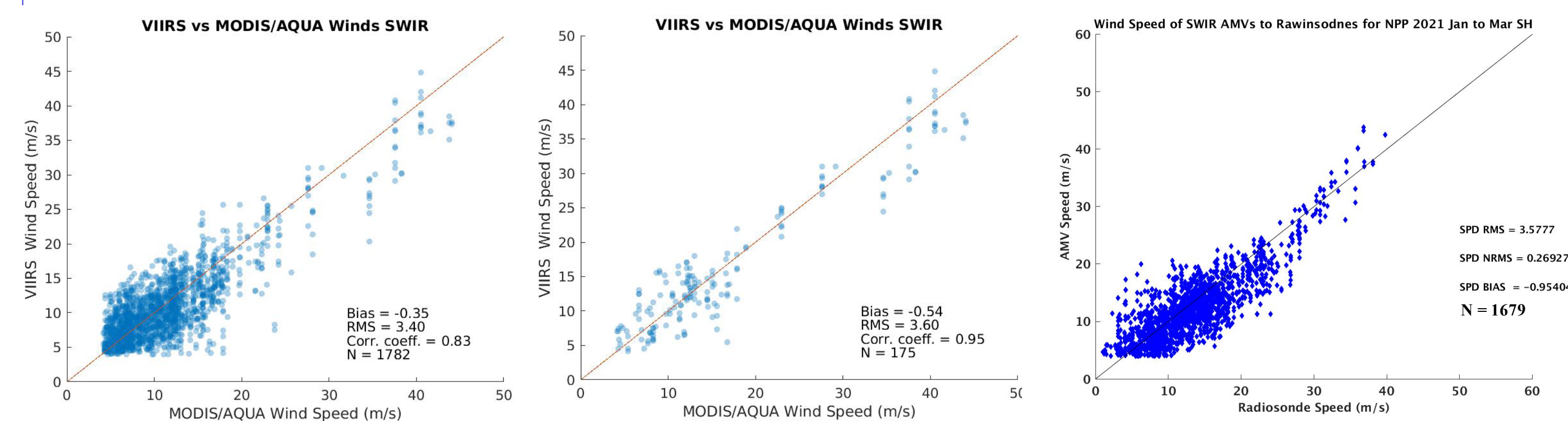
S-NPP VIIRS vs Aqua MODIS SWIR wind speed in the Antarctic for 18-23 February 2021. QI > 60 .
