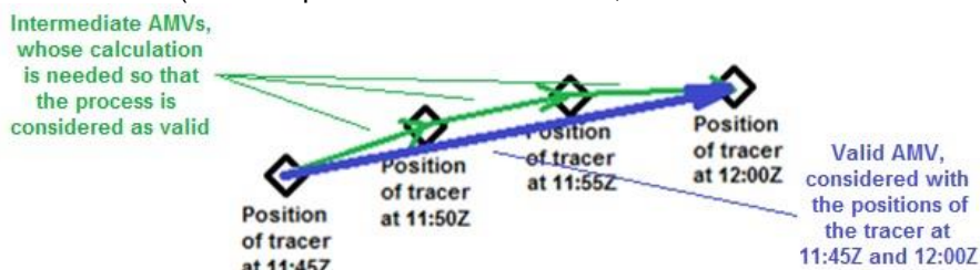
Figure 8: Schema for the AMV calculation, using the “mixed scanning processing”, with Rapid scan and Nominal scan with MSG satellites. The tracking process of the tracer is verified every 5 minutes, while the AMV is calculated considering the positions of the tracer every 15 minutes.
