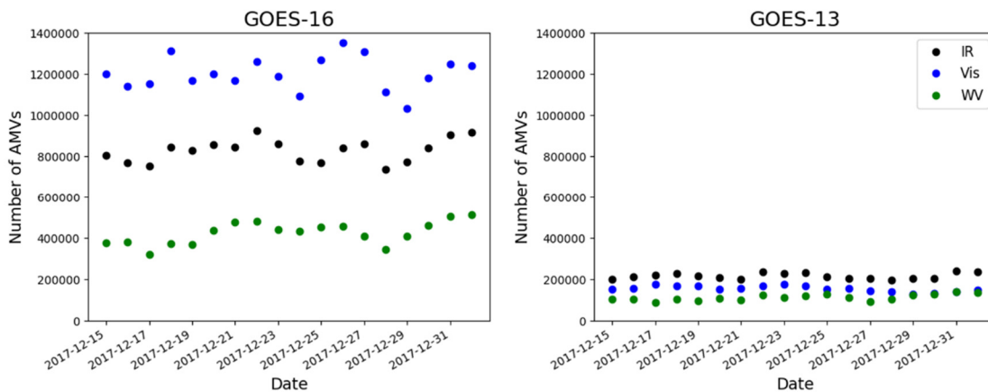
Figure 1 Time series showing the daily number of AMVs derived for the infrared, visible and water vapour channels on GOES-16 (left) and GOES-13 (right). Data are from 15 th Dec 2017 - 1 st Jan 2018 and no prior screening has been applied.
