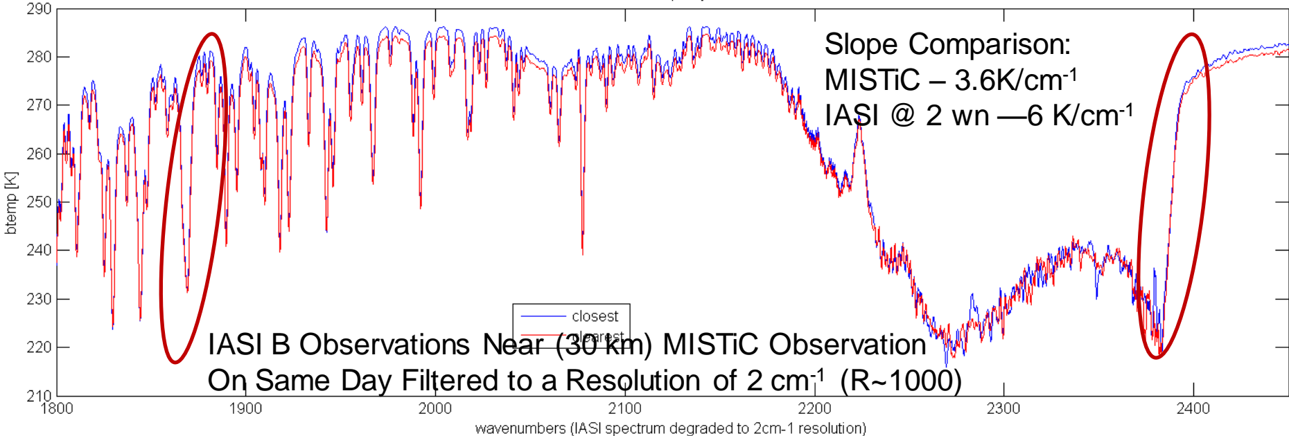
iasi.20171204.363.MetOp.day near W120.2 +33.7
