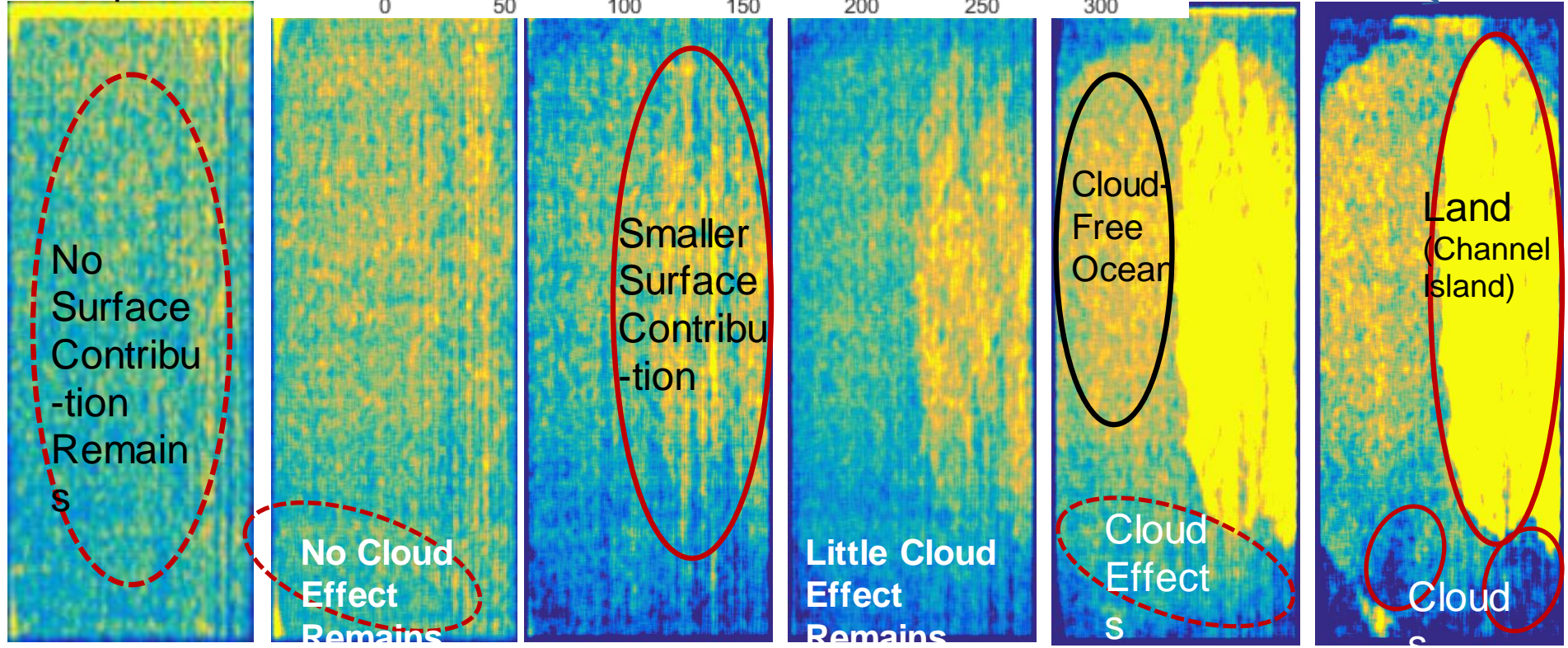
Selected CO 2 (Temperature)-Band Channels
