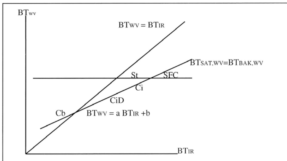
Fig. 1 Scatter diagram of IR and WV BTs at different cloud conditions (from Xu and Zhang, 1996)
