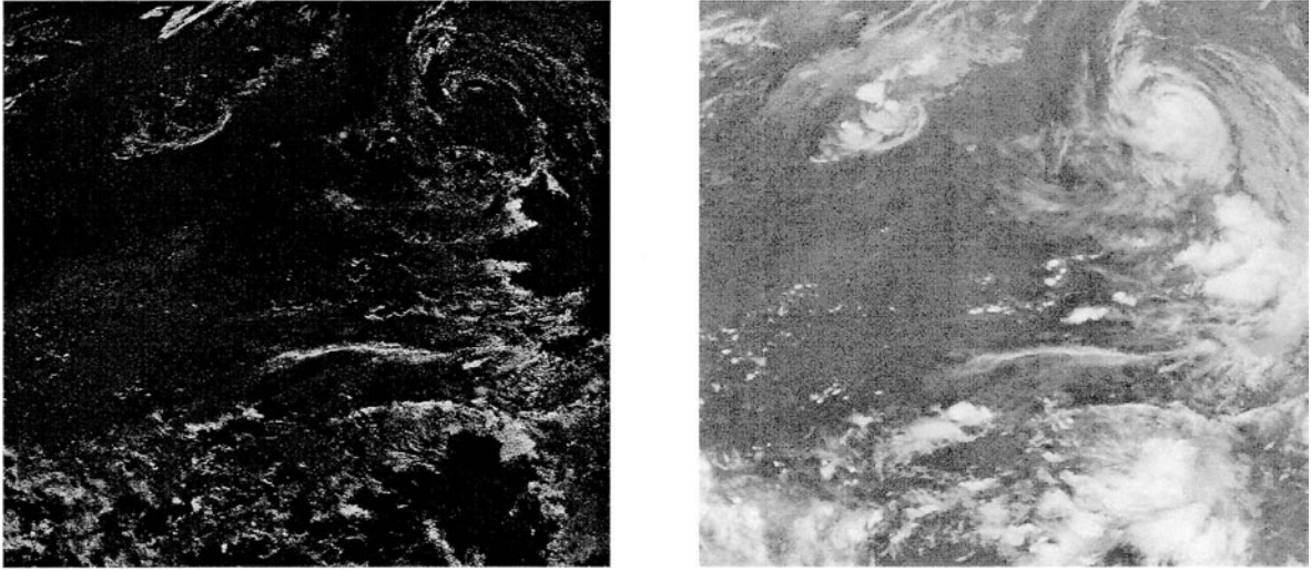
Fig 6 BTD_{IR}(a) and IR(b) images for GMS-5 at 17z 03 Sept. 1998.
