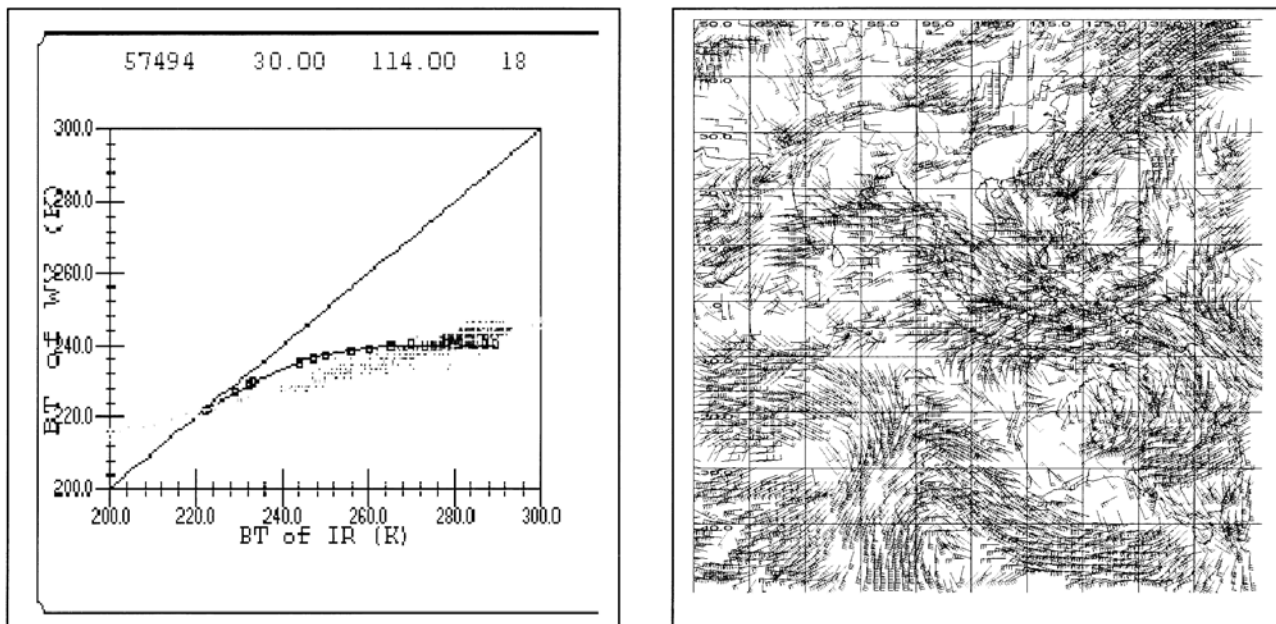
Fig. 8 Comparisons of IR / WV measurement relationship for opaque clouds with different hypothesis.
