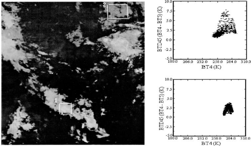
Fig. 7 a IR image from NOAA at 2036z 2 Aug. 1993, b Scatter diagram of BTD_{IR} - BT_{IR} for high cloud region 1 in Fig. 7 a, c Scatter diagram of BTD_{IR} - BT for low cloud region 2 in Fig. 7 a.
