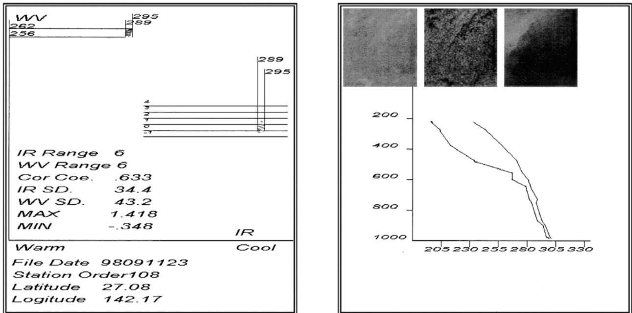
Fig. 5 scatter diagrams of IR / WV(up left) and IR /BTD IR (down right) measurements (a), radiosonde diagram and IR (left), BTD IR (middle) WV (right) images (b) for a GMS-5 tracer at 27.08 N 142.17 E, 00z 12 Sept. 1998.
