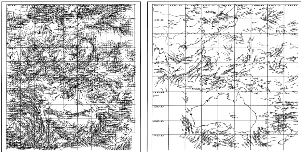
Fig. 10 GMS CMWs from NSMC at 00z 13 Sept. 1998.(left)
