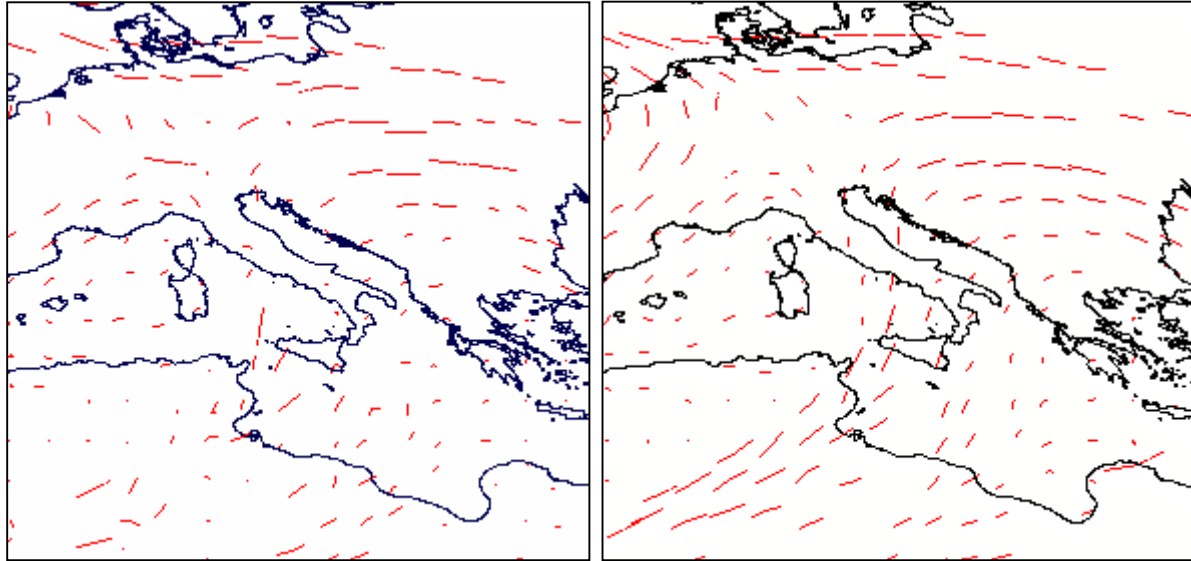
Figure 4. Infrared winds (CMW-IR) derived from Meteosat imagery, March 6 th 2002, 0500 UTC. The rapid scan winds (right figure) clearly have a more coherent structure than the operational winds (left figure).
