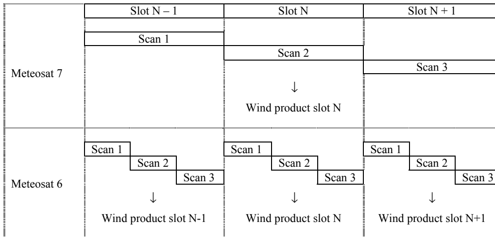
Figure 2. Schematic overview of full-earth (Meteosat-7) and rapid scan (Meteosat-6) wind product generation. A slot represents a 30 minute time interval.
