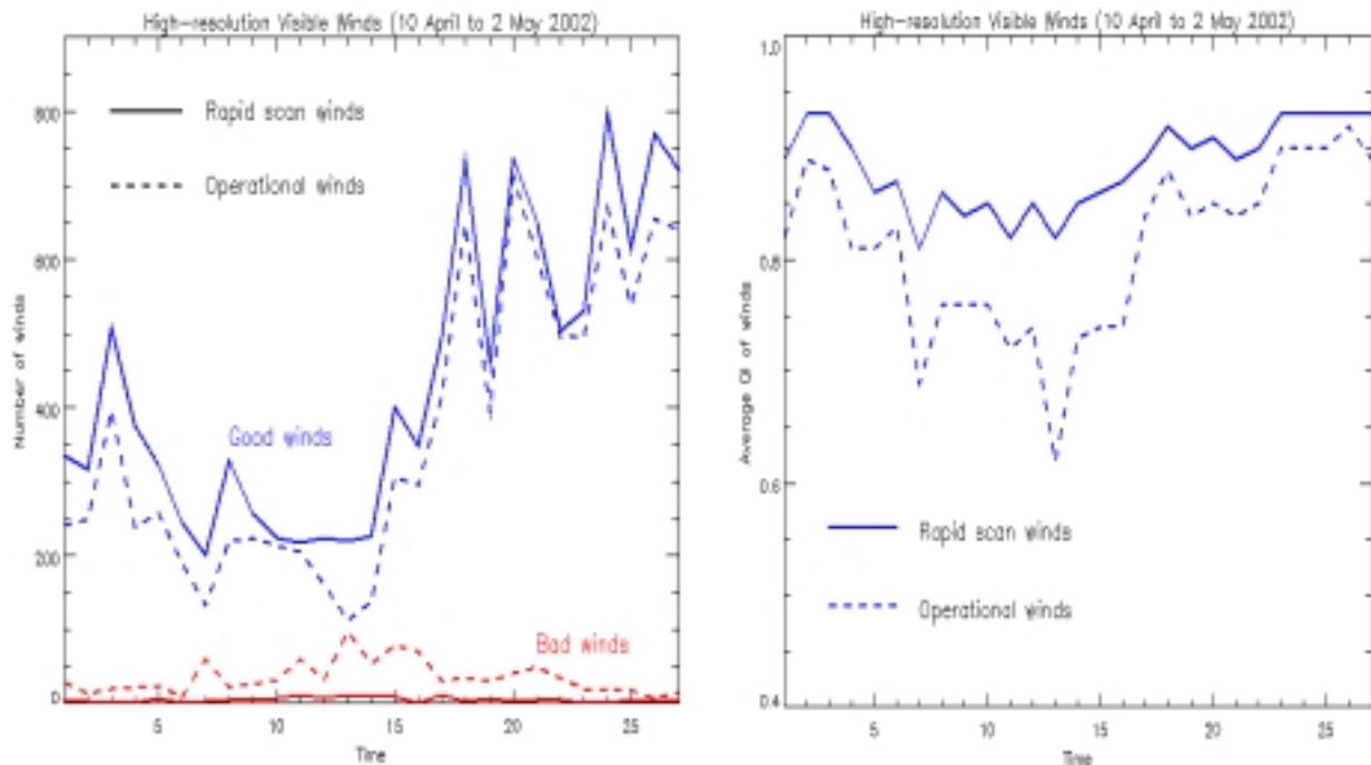
Figure 3. Number and quality of derived high-resolution visible winds as a function of time. The left picture shows both the number of very good winds ( QI \geq 0.9 ) and the number of poor winds ( QI < 0.3 ). The right picture shows the average Quality Indicator (QI) of the extracted winds. The numbers on the horizontal axis represent the comparison index number.
